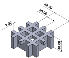
ISOMETRIC VIEW
