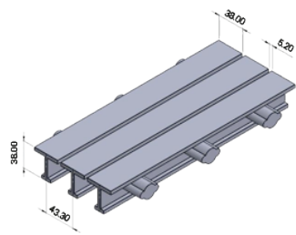
ISOMETRIC VIEW
